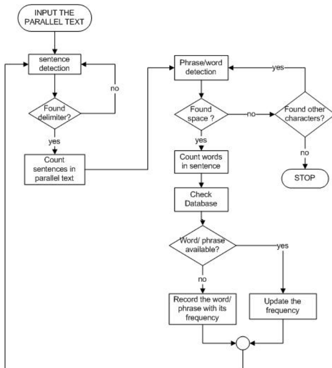
Fig. 3 The parsing process
