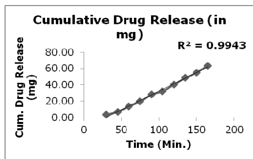
Fig. 2 Zero order model for drug release pattern
