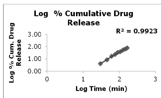
Fig. 4 Korsmeyer Peppas model for drug release pattern
