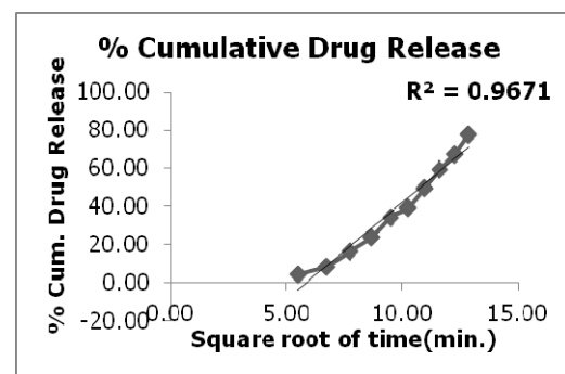
Fig. 5 Higuchi's model for drug release pattern
