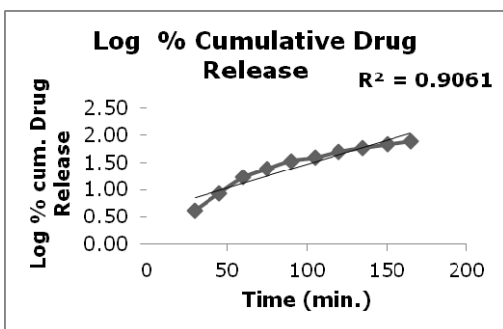
Fig. 3 First order model for drug release pattern
