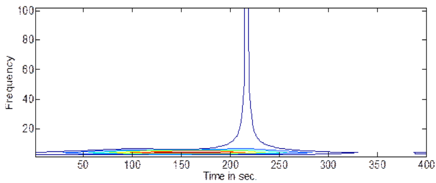
Fig. 8 S-matrix contour of swell signal
