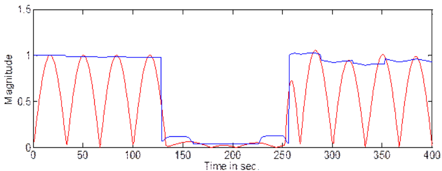
Fig. 4 Initial detection of voltage sag
