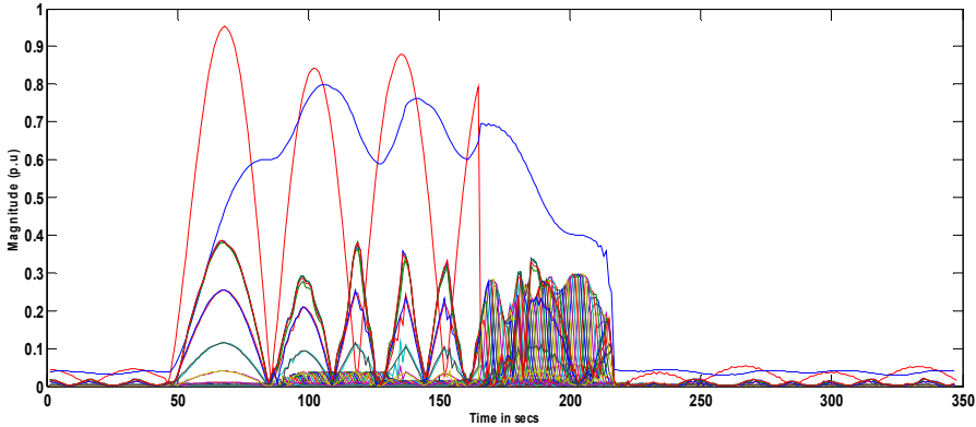
Fig. 10 Half cycle Windowing Technique (samples, N=64) with modified parameters (miw) for swell signal
