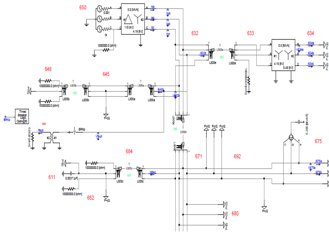
Fig. 1 IEEE 13 bus PSCAD simulation
