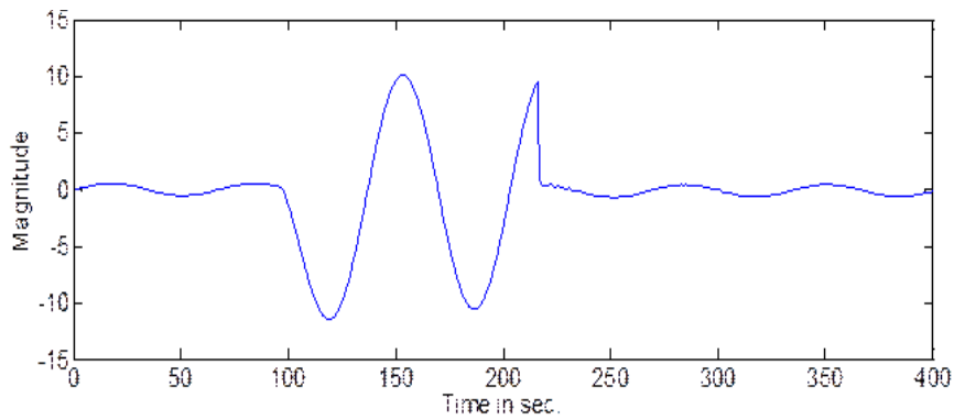
Fig. 7 Voltage swell signal
