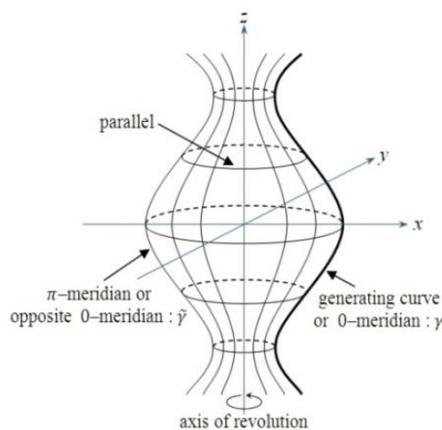
Fig. 1 Surface of revolution
