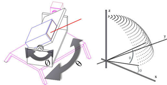
Fig. 1 Mechanical part of scanner and scanning area
