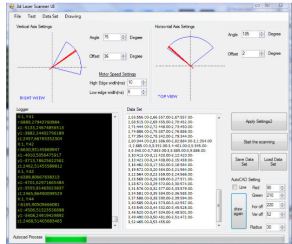
Fig. 4 Software User Interface
