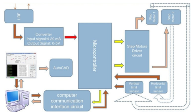
Fig. 2 Device modeling
