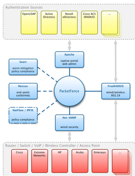
Fig. 2 PacketFence (Open source NAC) [2]
