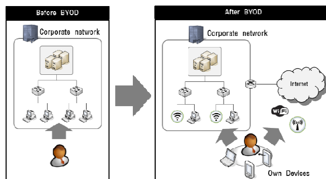
Fig. 1 BYOD Environment
