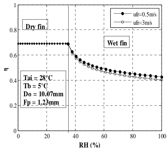
Fig. 4 Effect of frontal velocity on fin efficiency
