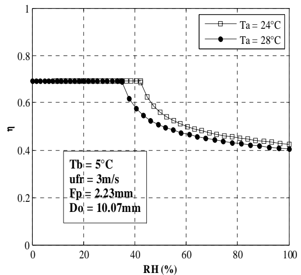
Fig. 7 Effect of air temperature on fin efficiency
