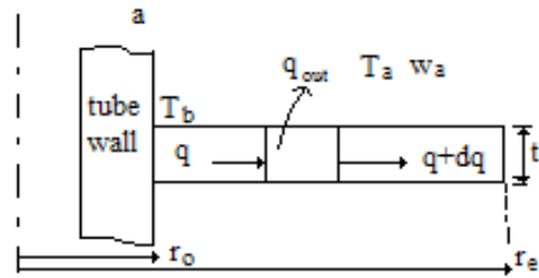
Fig. 1 Schematic Diagram of Circular fin
