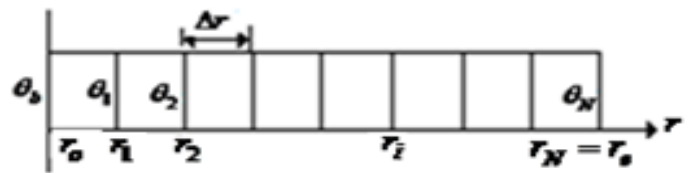
Fig. 2 Finite difference scheme for 1-D circular fin
