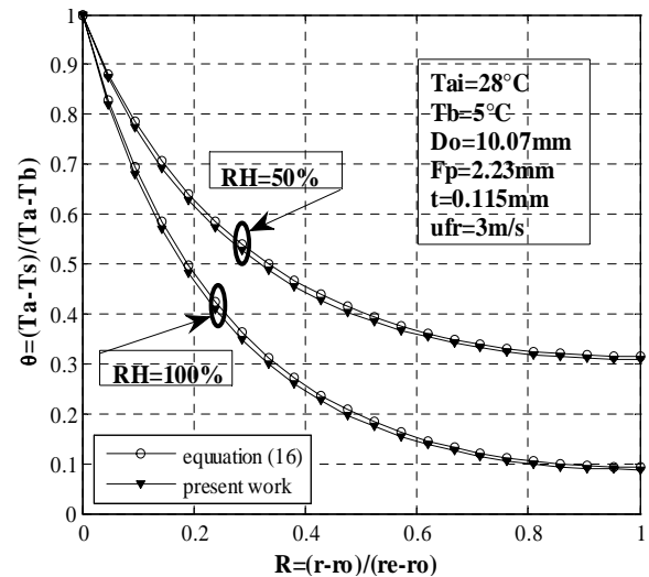
Fig. 3 Fin surface temperature comparison
