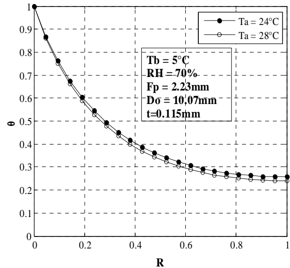
Fig. 6 Effect of air temperature on fin surface temperature
