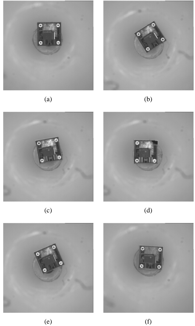
Fig. 3 Object image size= 800 \times 800 , model image size= 212 \times 212 . (a) Image for the model extraction; (b) Position (404.162, 345.419), rotation: 9.574, similarity: 0.856; (c) Position (373.935, 359.307), rotation: 357.294, similarity: 0.737; (d) Position (406.175, 319.089), rotation: 22.984, similarity: 0.962; (e) position (418.058, 310.604), rotation: 356.354, similarity: 0.905; (f) Position (417.678, 324.021), rotation: 31.636, similarity: 0.908
