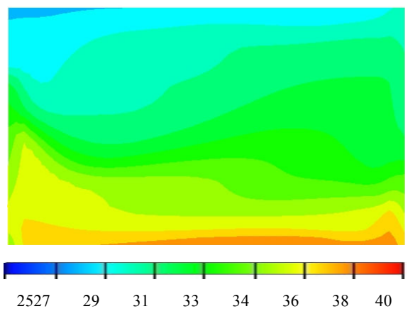
Fig. 9 Relative humidity on plane at Z=1.5 m for case A12R50 at t_{in}=21^{\circ}\text{C}
