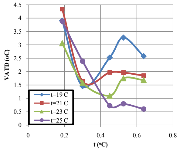
Fig. 12 Vertical air temperature difference between 0.1m and 1.1m above floor at \text{RH}_{in}=50\%
