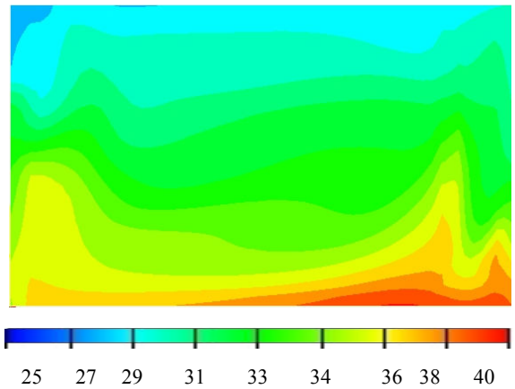
Fig. 8 Relative humidity on plane at Z=0.75 m for case A12R50 at t_{in}=21^{\circ}\text{C}
