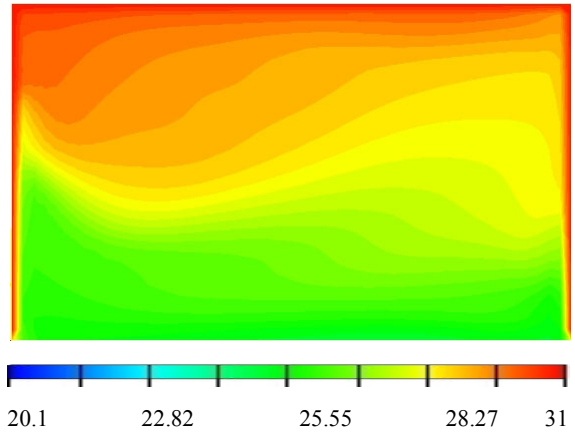
Fig. 7 Temperature contour on plane at Z=1.5 m for case A12R50 at t_{in}=21^{\circ}\text{C}
