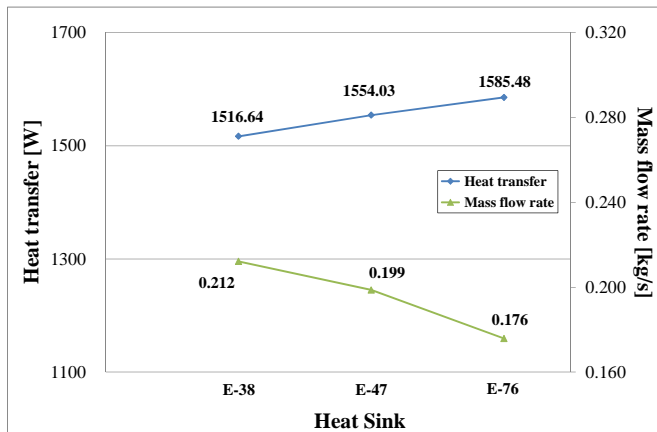
Fig. 6 Heat transfers thru the heat sinks and the mass flow rates of the four heat sink
