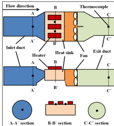
Fig. 1 A schematic of the experimental setup
