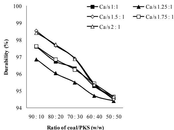
Fig. 4 Durability of bio-briquettes using scallop shell desulfurizer
