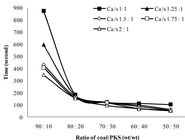
Fig. 6 Water resistance of bio-briquettes using lime desulfurizer
