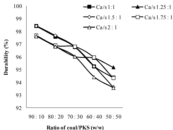
Fig. 5 Durability of bio-briquettes using green mussel shell desulfurizer
