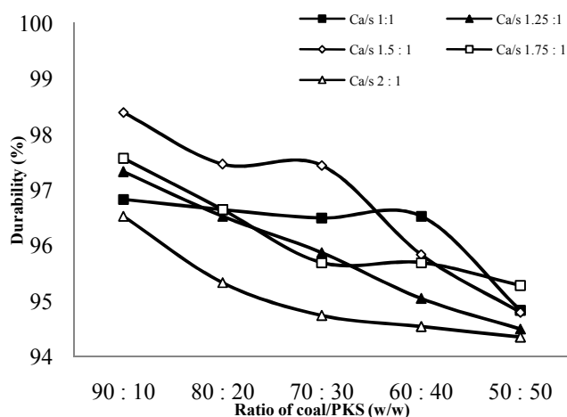
Fig. 2 Durability of bio-briquettes using lime desulfurizer
