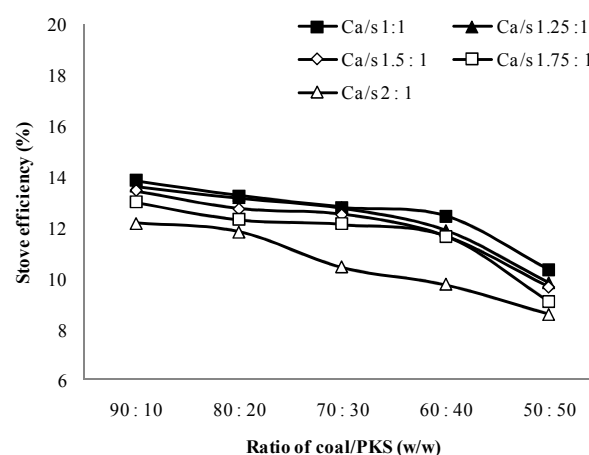
Fig. 8 Stove efficiency for bio-briquettes using lime desulfurizer
