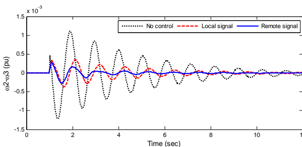
Fig. 22 Local mode of oscillation for small disturbance
