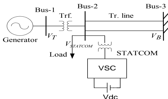
Fig. 1 Single-machine infinite-bus power system with STATCOM
