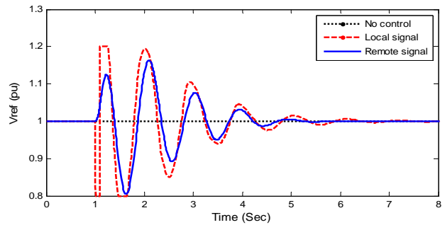
Fig. 11 Vref voltage with Light loading
