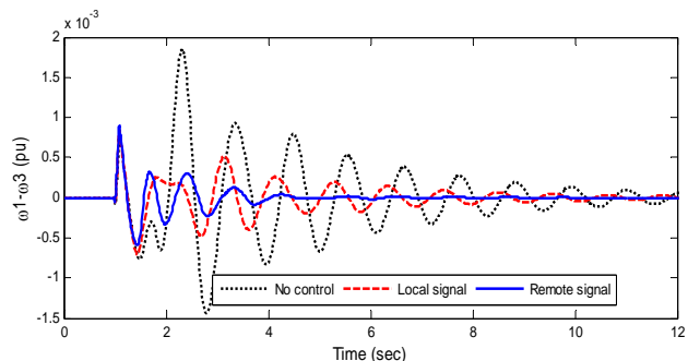
Fig. 16 Inter-area mode of oscillation for 5 cycle 3-phase fault disturbance
