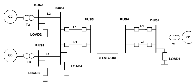
Fig. 15 Three machine power system with STATCOM
