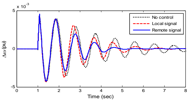
Fig. 9 Speed deviation response for 5 cycle 3-ph fault in transmission line with Light loading
