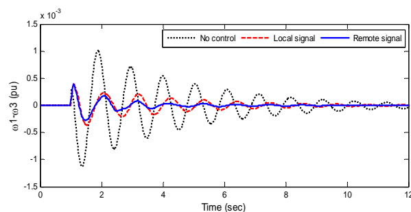
Fig. 21 Inter-area mode of oscillation for small disturbance
