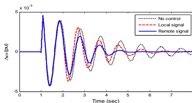
Fig. 5 Speed deviation response for 5 cycle 3-ph fault in transmission line with nominal loading
