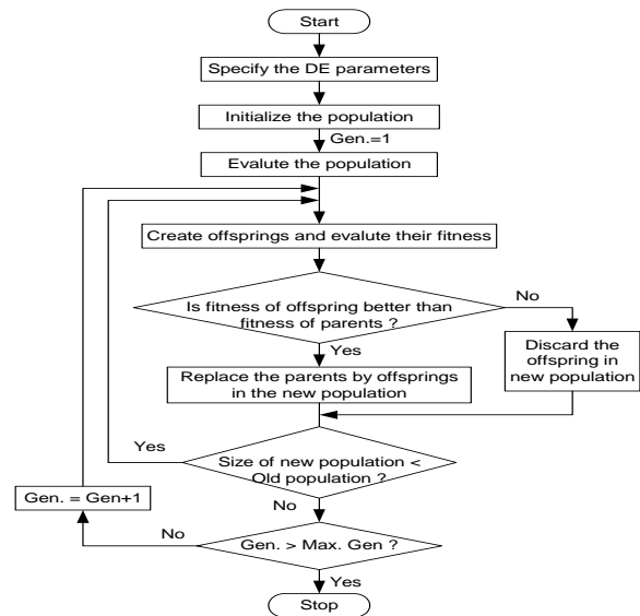
Fig. 4 Flow chart of proposed DE optimization approach
