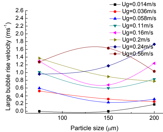
(a) Single large bubble velocity
