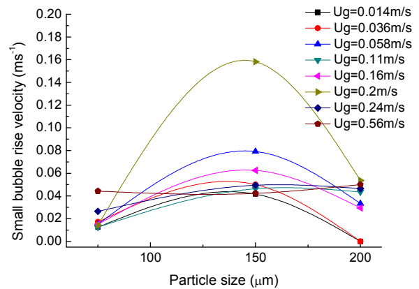
(b) Single small bubble velocity
