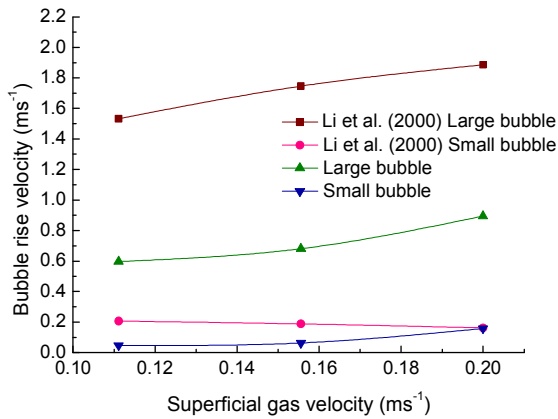
Fig. 4 Bubble rise velocity profiles of large bubble and small bubble
