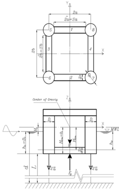
Fig. 2 The Square TLP (plan and elevation)
