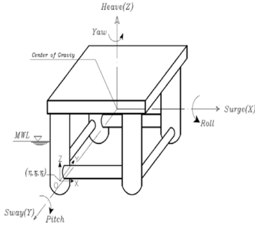
Fig. 1 The global and local coordinate system of TLP
