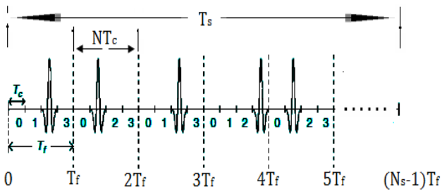
Fig. 1 TH-UWB signal
