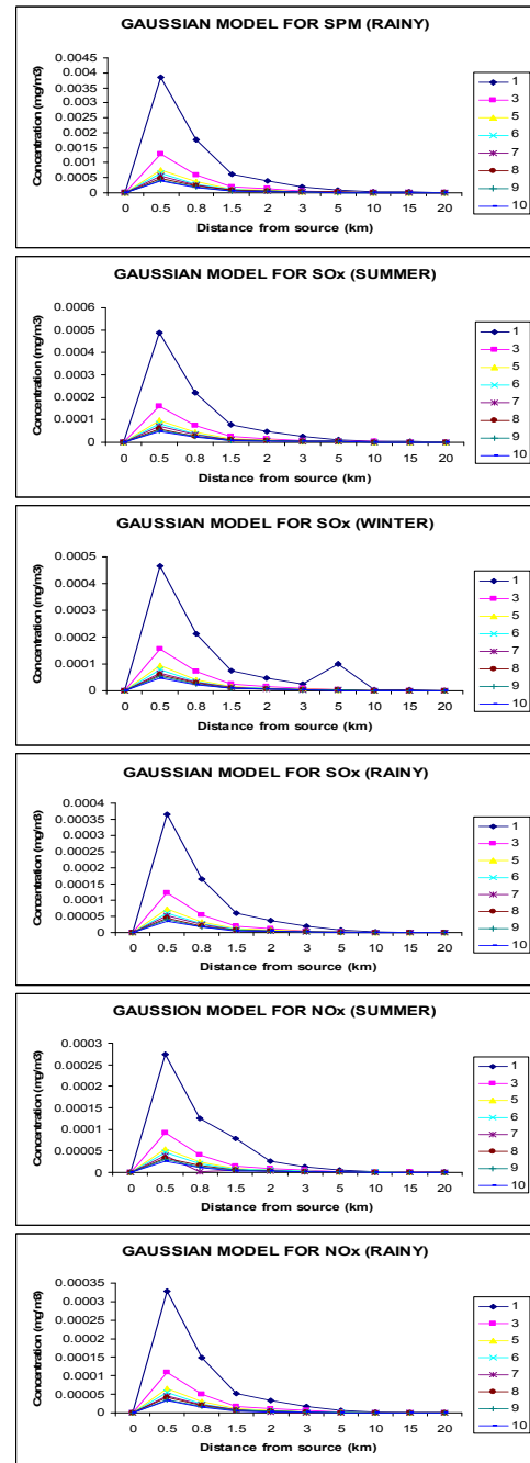
Fig. 3 Gaussian model for different season and pollutants
