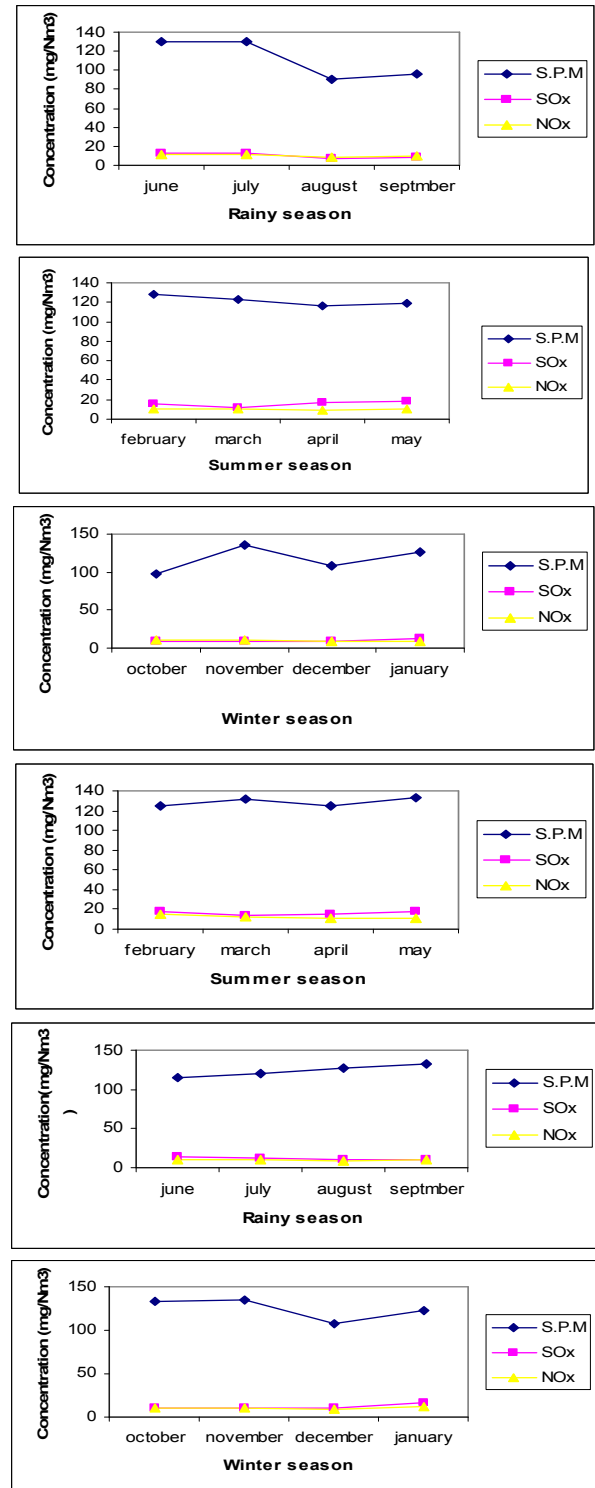
Fig. 1 Stack analysis of NRE coke for different seasons and different stack
