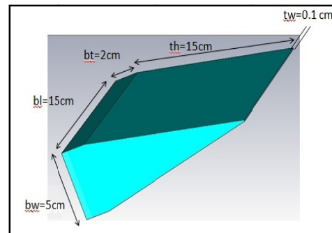
Fig. 6 Design of truncated wedge microwave absorber
