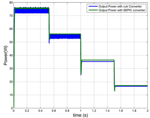
Fig. 11 Power at constant temperature of 25°C with step changes of irradiance
