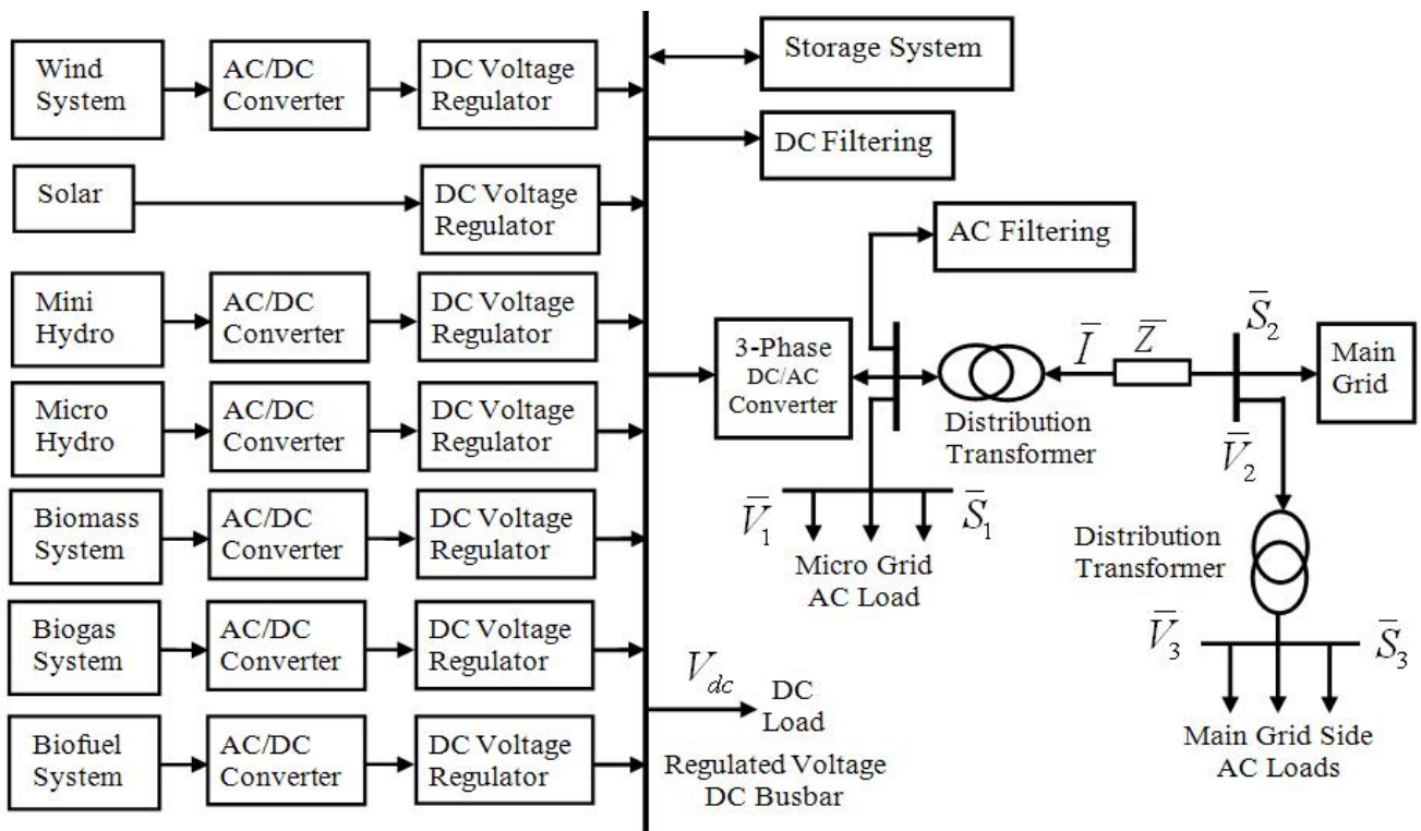
Fig. 1 Configuration of the multisource microgrid [8]
