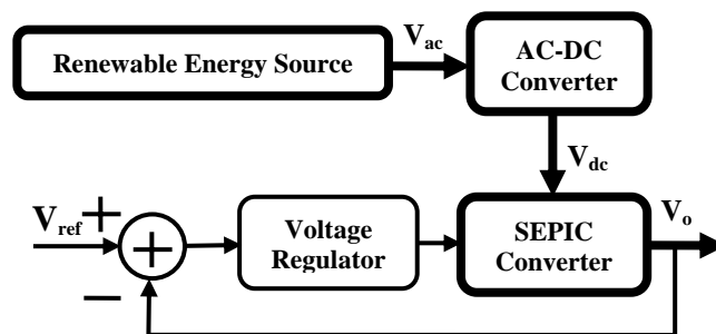
Fig. 3 DC voltage regulator based on SEPIC converter
