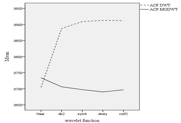
Fig. 2 ACF of DWT and MODWT
