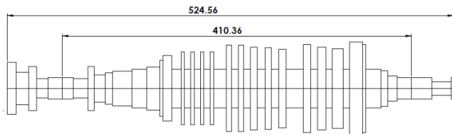
Fig. 3 Geometry of the rotor (length in cm)
