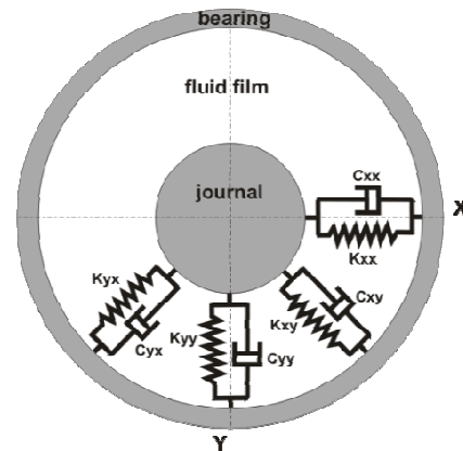
Fig. 2 Model of fluid-film bearing
