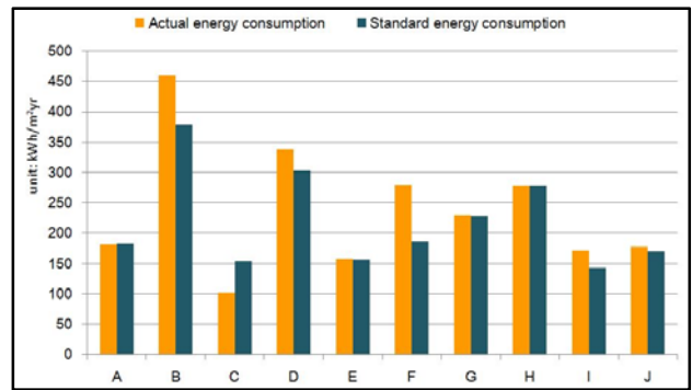
Fig. 9 Comparison actual and standard energy consumption
