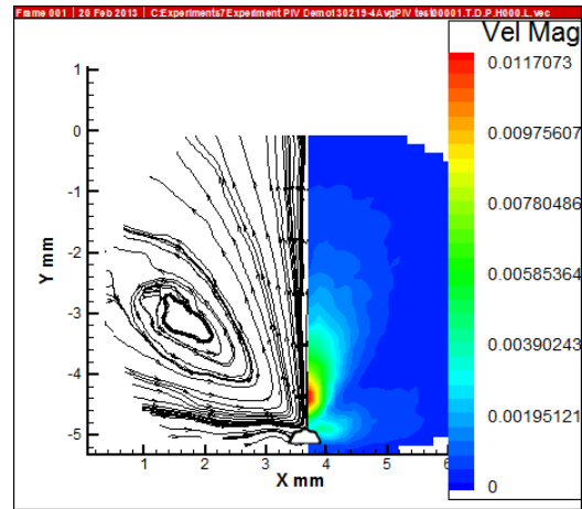
Fig. 4 The velocity fields of steady streaming flow around an oscillating bubble measured by the micro-PIV. The left panel shows streamlines and the right panel shows velocity contours
