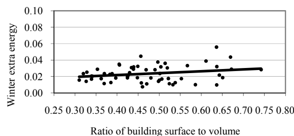
Fig. 1 Winter extra energy consumptions and ratios of building surface to volume of sample schools
