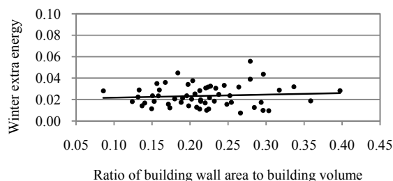
Fig. 10 Winter extra energy and ratio of building wall area to building volume
