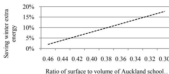
Fig. 2 Savings in mean winter extra energy with decreasing mean ratio of building surface to volume of Auckland school buildings
