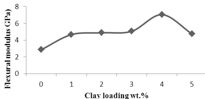
Fig. 10 The effect of clay loading on flexural modulus [5]
