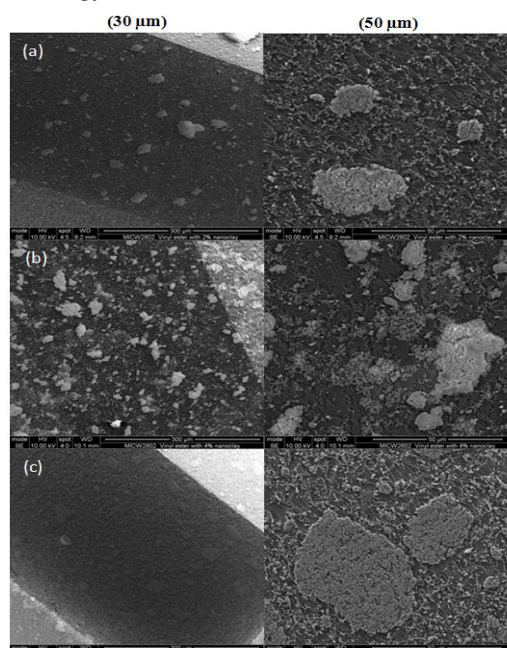
Fig. 4 SEM images at 30 \mu m and 50 \mu m of (a) 2 wt.%, (b) 4 wt.% and (c) 5 wt.% nanocomposites [5]
