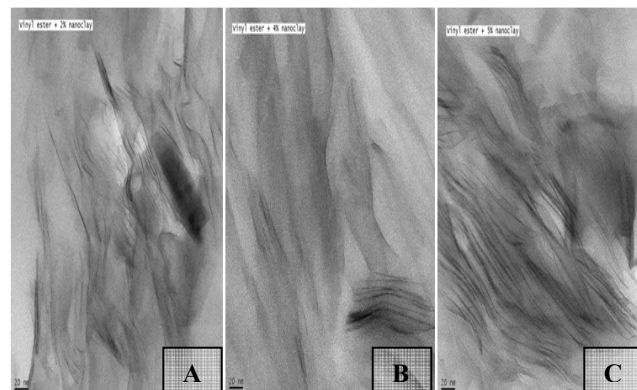
Fig. 6 TEM micrographs at 20 nm magnification of (a) 2 wt.%, (b) 4 wt.% and (c) 5 wt.% nanocomposites [5]
