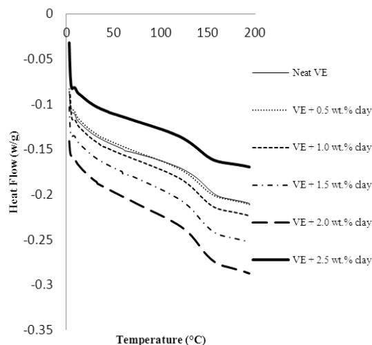
Fig. 17 DSC curve of the neat vinyl ester and the corresponding nanocomposites [4]
