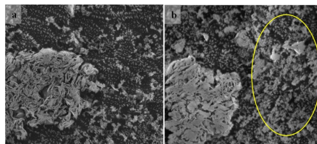
Fig. 3 SEM images at 50 \mu m of (a) 1 wt.% and (b) 2.5 wt.% nanocomposites [4]
