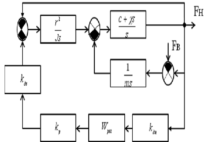
Fig. 4 Block diagram of SSRT
