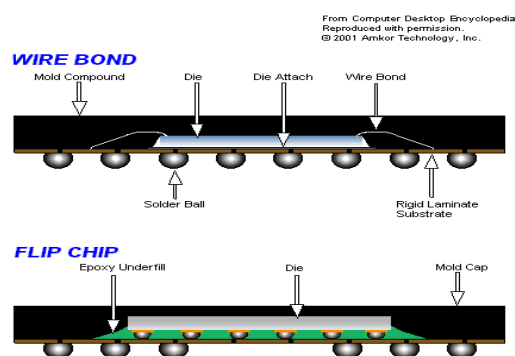
Fig. 1 The difference between wire bond chip and flip chip
