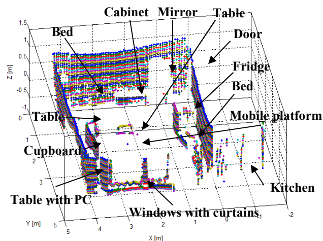
Fig. 13 3D vector map of room – daylight
