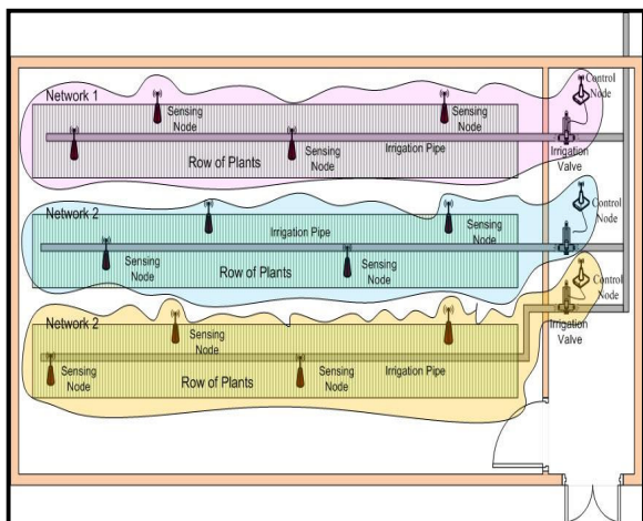
Fig. 1 Overall system layout
