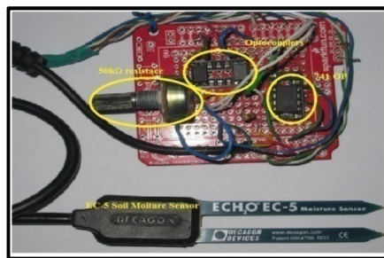
Fig. 4 Practical excitation circuit for EC-5 sensor
