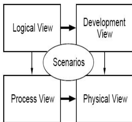
Fig. 3 "4+1 View Model"
