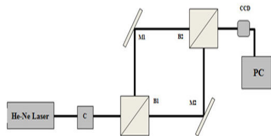
Fig. 1 Schematics of Mach-Zehnder interferometer
