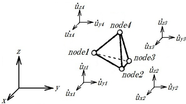
Fig. 2 Relationship between particle velocity and strain
