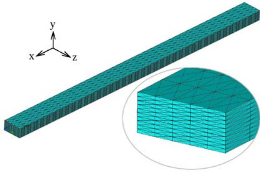
Fig. 3 Three-dimensional slit model for the FEM
