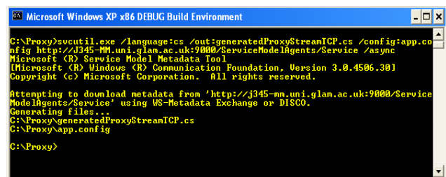
Fig. 11 The Svcutil.exe Command
