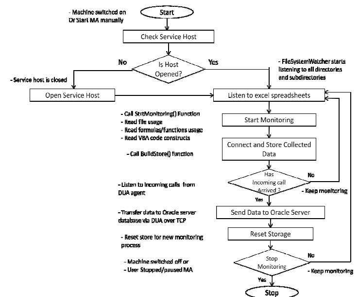
Fig. 4 The Basic Algorithm of The MA
