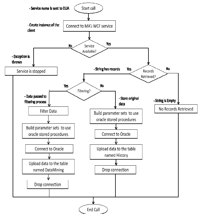
Fig. 14 The Basic Algorithm of the DUA
