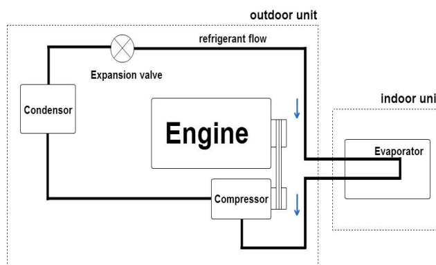
Fig. 1 Outline of GHP system (cooling cycle)
