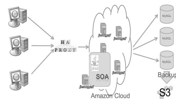
Fig. 6 Architecture of Playfish
