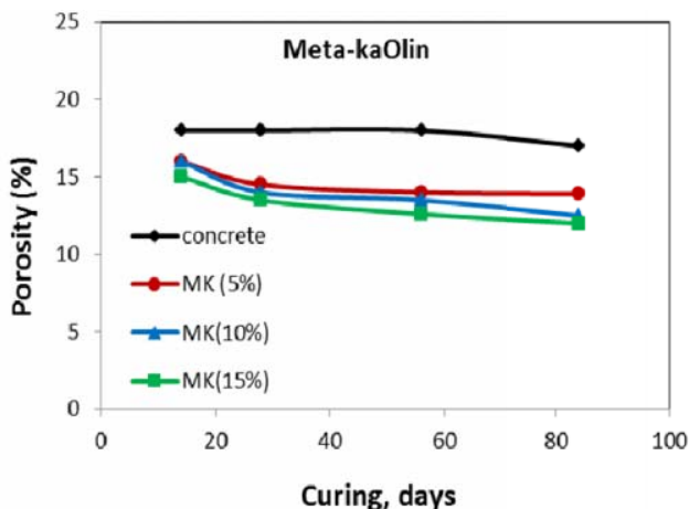
Fig. 3 Porosity decrease of specimens during concrete curing
