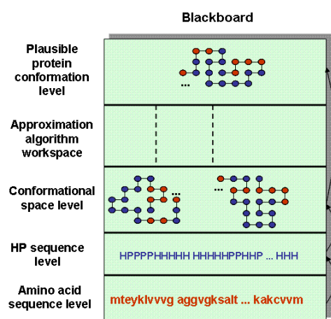
Fig. 2 Defined blackboard steps in the bioinformatics platform
