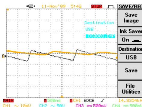
Fig. 10 Inductor current and input current waveforms
