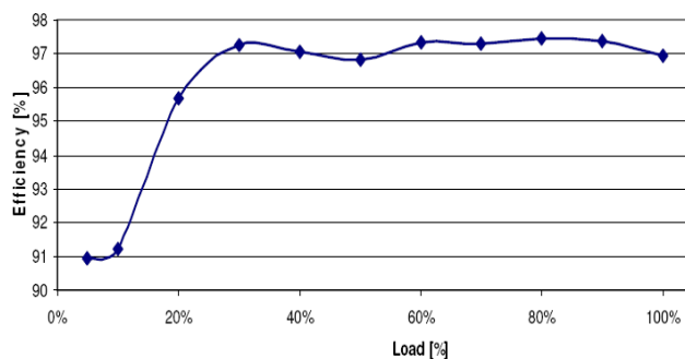
Fig. 13 Converter's overall efficiency
