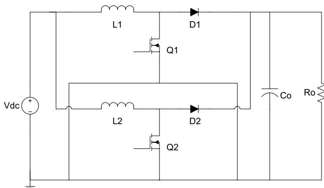
Fig. 2 Multiphase boost topology
