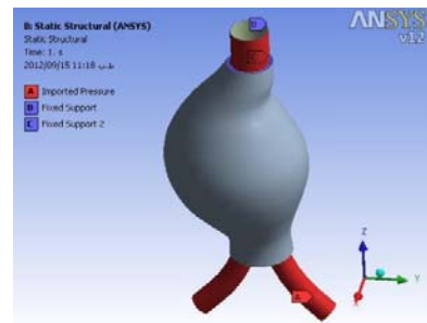
Fig. 4 Applied boundary condition on model
