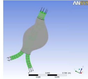
Fig. 2 Inlet and outlet fluid direction in graft
