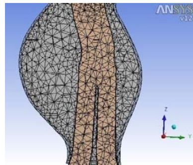
Fig. 3 Generated mesh on ANSYS CFX model
