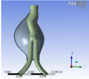
Fig. 1 Graft, Aneurysm sac and wall
