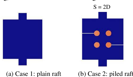
Fig. 1 Two cases were conducted in centrifuge tests
