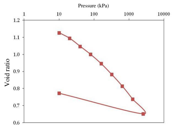
Fig. 8 e -logP curve of clay
