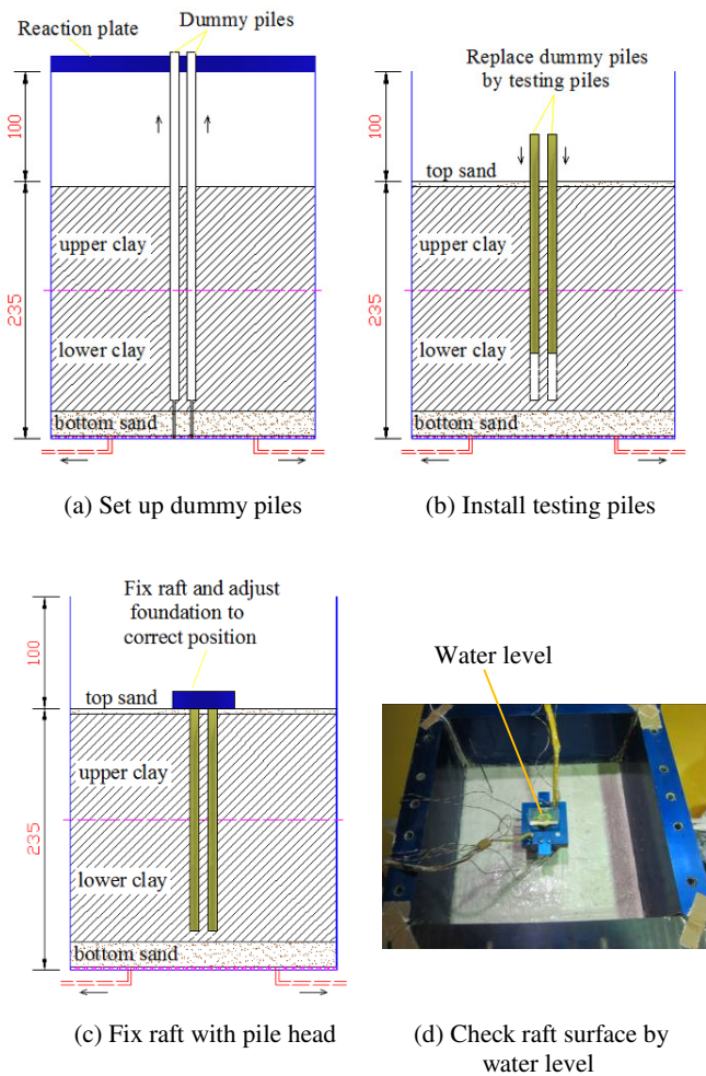
Fig. 10 Installation of piled raft model
