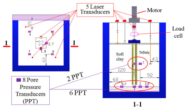
Fig. 4 Instrumentations of ground model
