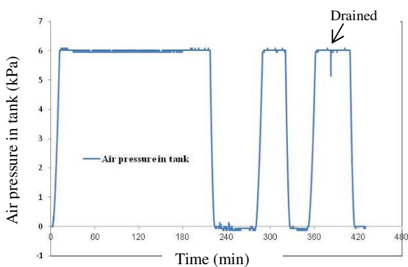
Fig. 21 The variation of air pressure in tank with time in case 1
