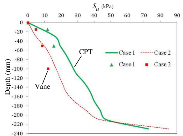
Fig.7 Shear strength of soil models
