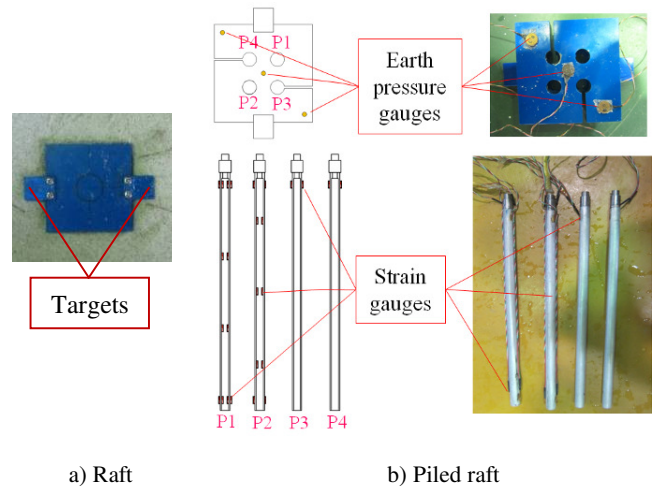
Fig. 3 Instrumentations of foundation models
