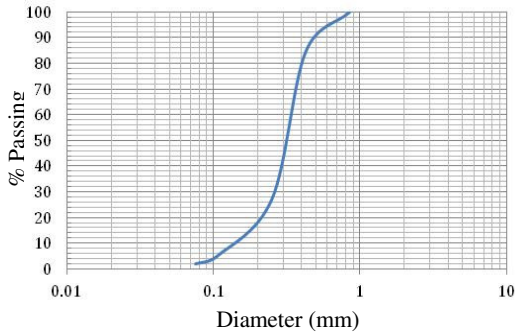
Fig. 9 Sieve analysis result of silica sand
