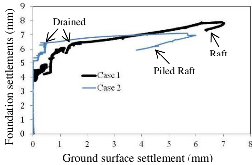
Fig. 16 Foundation settlements versus ground surface settlement
