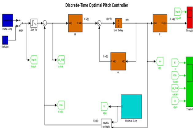
Fig. 5 Simulated model in Simulink
