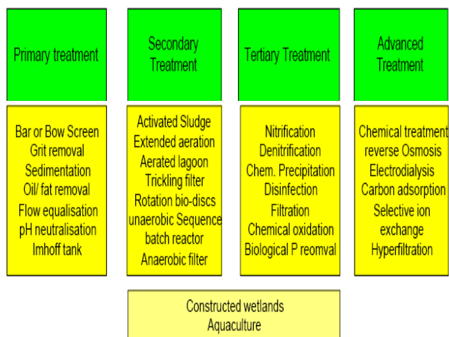
Fig. 2 Wastewater treatment categories and technologies
