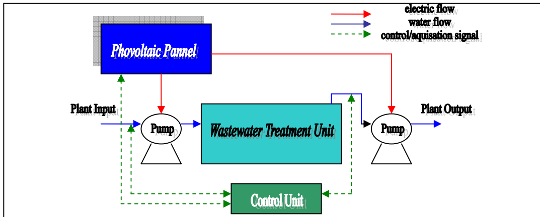
Fig. 3 Small-Scale Wastewater Treatment Plants
