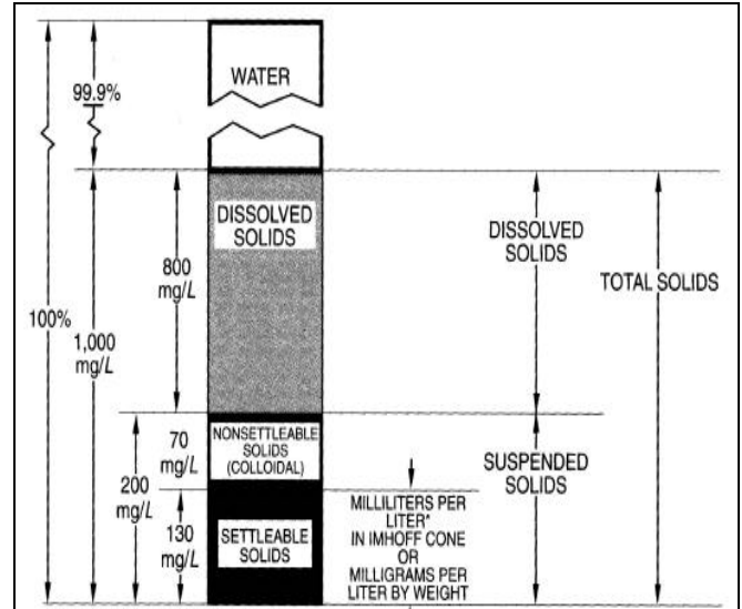
Fig. 1 Composition of solids in wastewater
