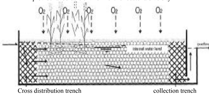
Fig. 5 Horizontal Gravel Filter
