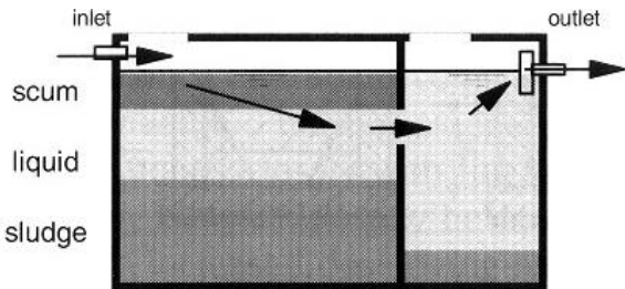
Fig. 4 Septic Tank
