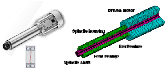
Fig. 3 High speed engraving spindle unit and finite element model, including the housing, shaft and bearings.
