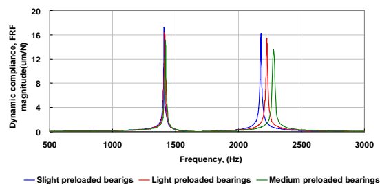
Fig. 6 Computed FRFs of the spindle system equipped with bearings at different preload amounts.
