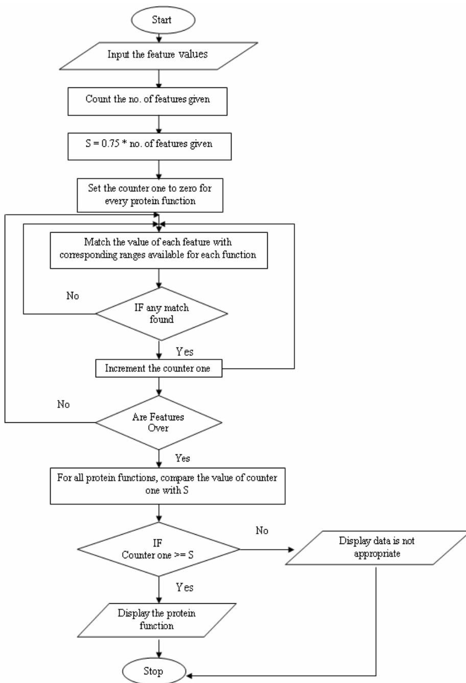
Fig. 2 Working Model for HPF predictor
