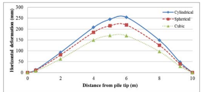
Fig. 8 Comparison of horizontal pile deformation for different explosive shapes
