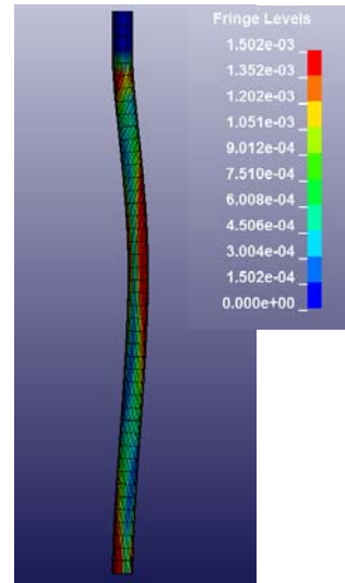
Fig. 7 Effective stress on the pile at 0.75s
