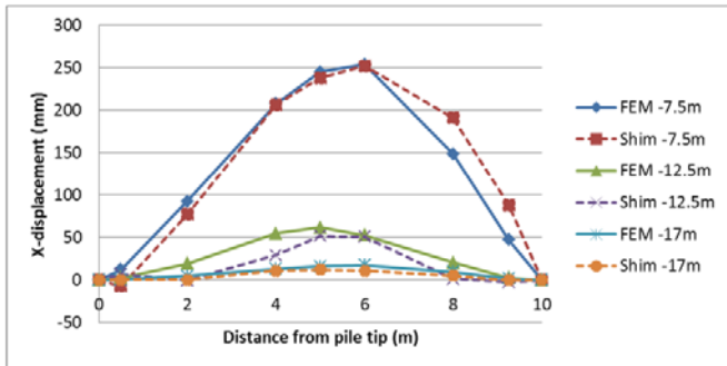
Fig. 6 Comparison of horizontal pile deformation
