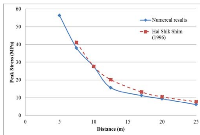
Fig. 4 Comparison of peak stresses
