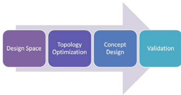
Fig. 9 Modified design cycle of Fuselage
