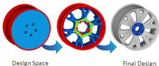
Fig. 1 Figure illustrating Topology Optimization
