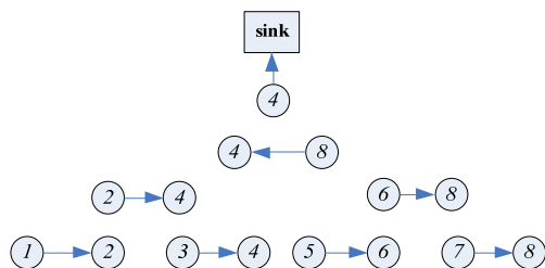
Fig. 3 Chain in PEGASIS
