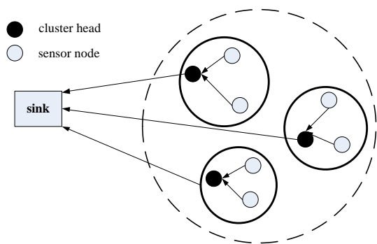
Fig. 2 Network structure of LEACH
