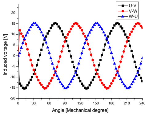
Fig. 2 Calculated back EMF waveform @ 10,000rpm
