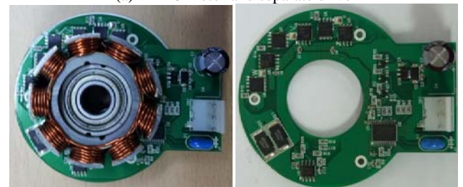
(b) BLDC motor and integrated drive
