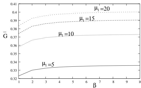
Fig. 8. Effect of \mu_1 on \bar{G} for H^* = 4.0 , M = 5.0 , \alpha = 1.0 and \epsilon = 0.2 .
