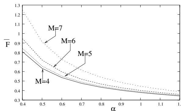
Fig. 3. Effect of \bar{M} on F for H = 4.0 , \mu = 10.0 and \epsilon = 0.2 .
