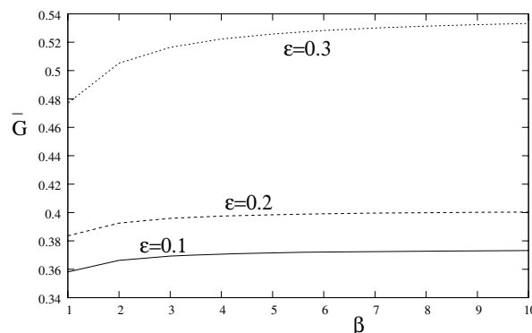
Fig. 9. Effect of \epsilon on \bar{G} for H^* = 4.0 , M = 5.0 , \mu_1 = 10.0 , and \alpha = 1.0 .
