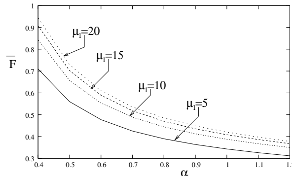
Fig. 4. Effect of \bar{\mu} on F for H = 4.0 , M = 5.0 and \epsilon = 0.2 .
