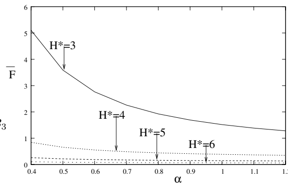
Fig. 2. Effect* of \bar{H} on F for M = 5.0 , \mu = 10.0 and \epsilon = 0.2 .
