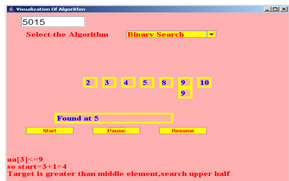
Fig. 6 Binary search- Element found
